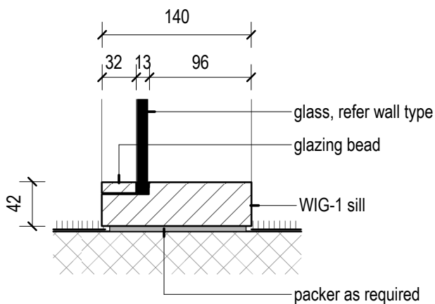
1 WIG-1 Sill Detail 1 : 5
