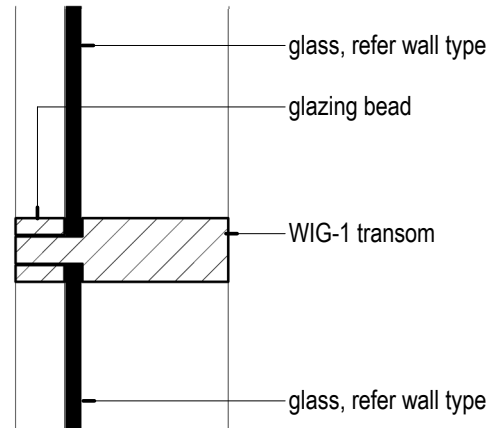
2 WIG-1 Transom Detail 1 : 5
